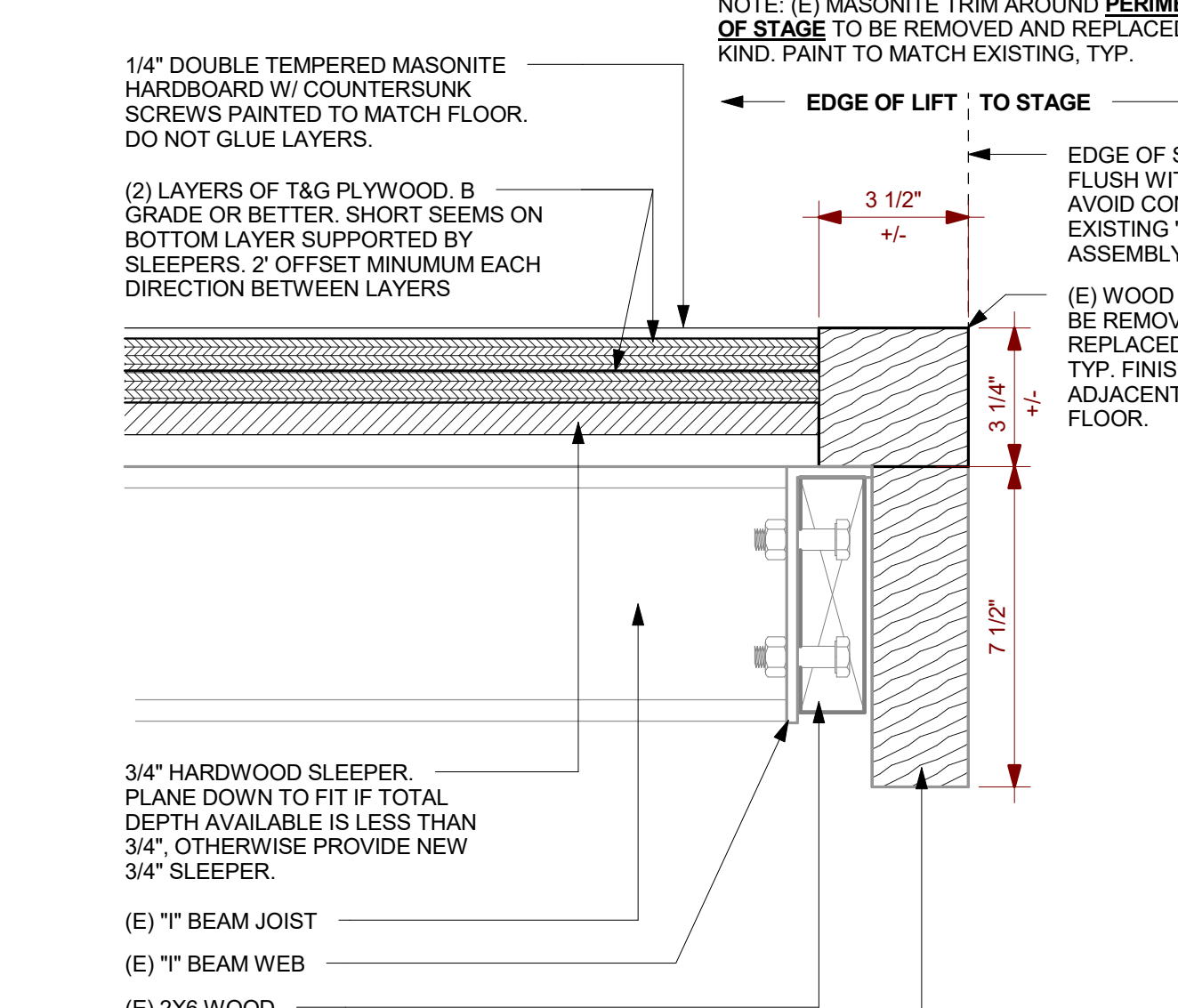
8 STAGE LIFT DETAIL B SCALE: 3" = 1'-0"
