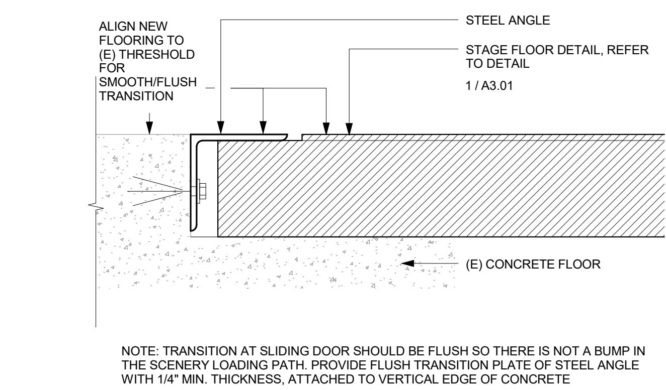
9 STAGE FLOOR TO CONCRETE TRANSITION SCALE: 3" = 1'-0"
