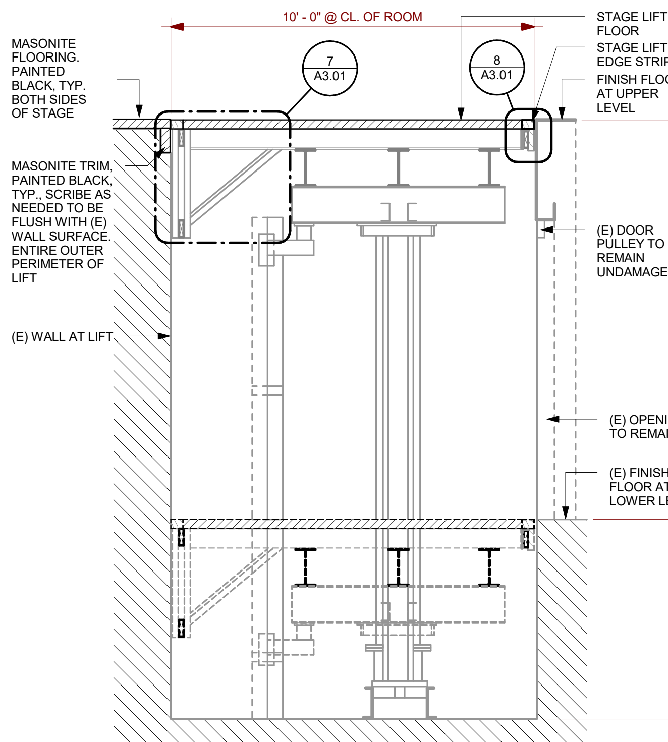
6 STAGE LIFT SECTION SCALE: 3/8" = 1'-0"
