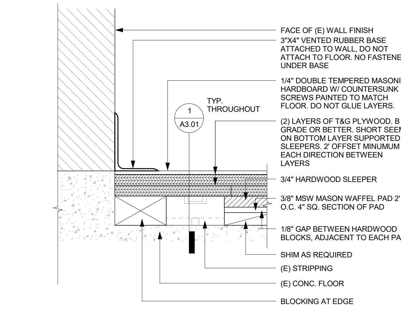
5 STAGE FLOOR DETAIL AT WALL SCALE: 3" = 1'-0"
