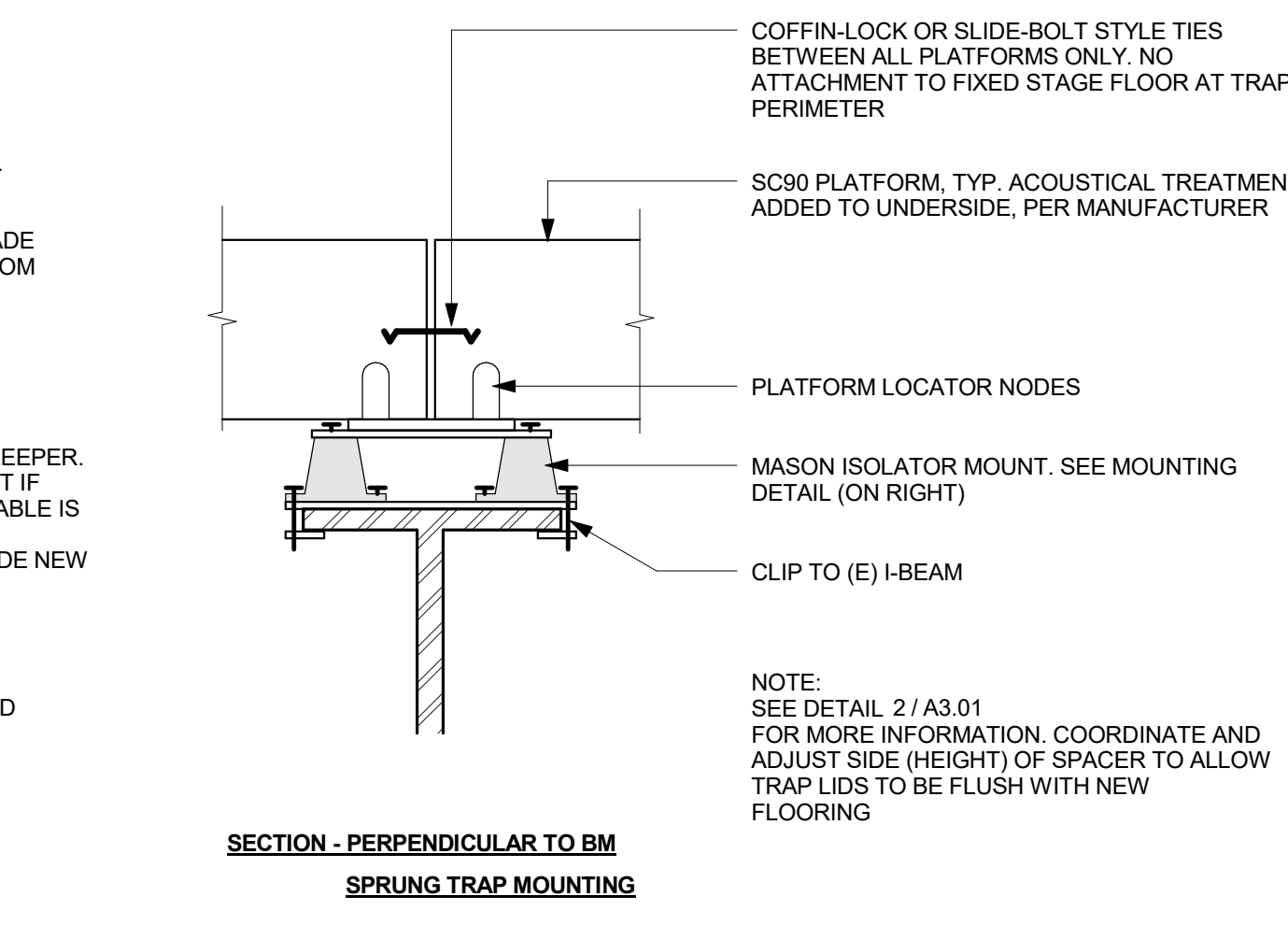
3 STAGE TRAP SECTION A SCALE: 3" = 1'-0"
