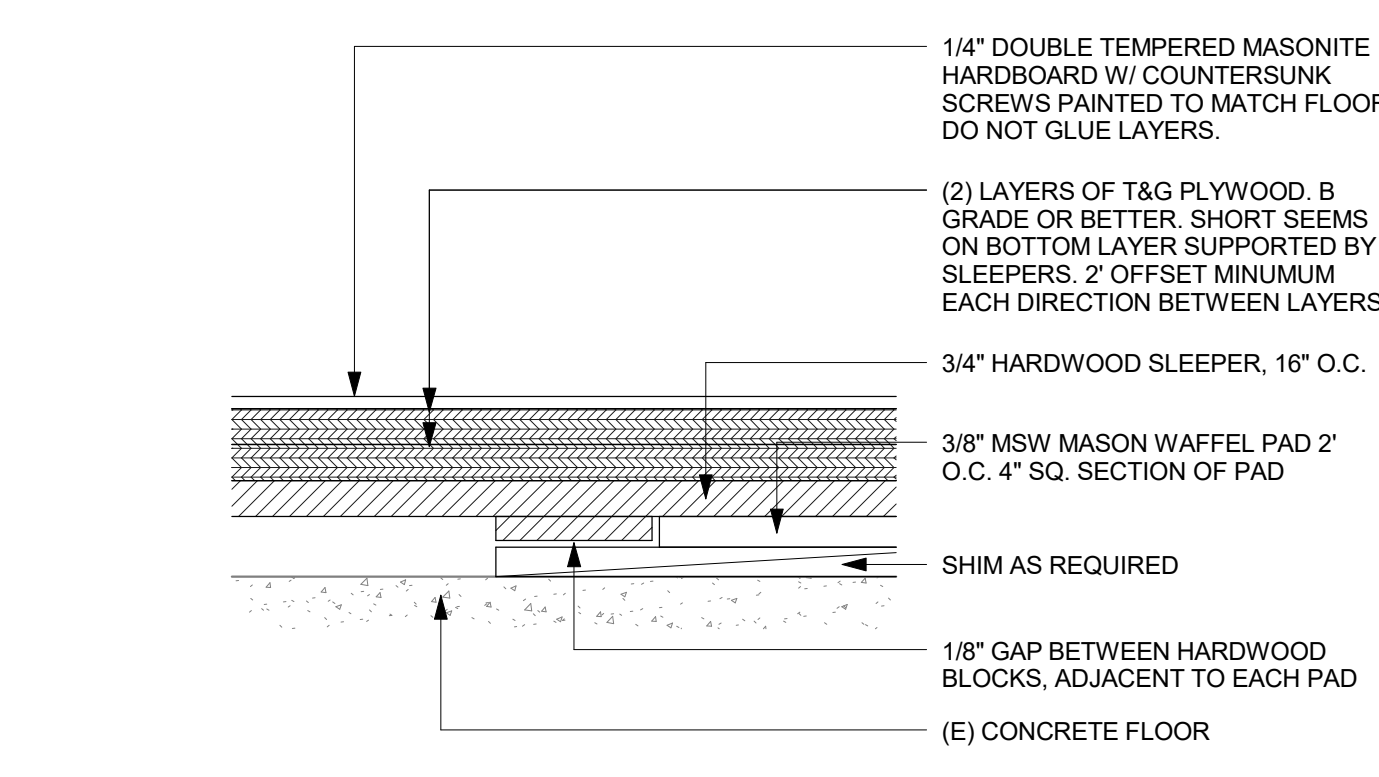
1 STAGE FLOOR DETAIL SCALE: 3" = 1'-0"
