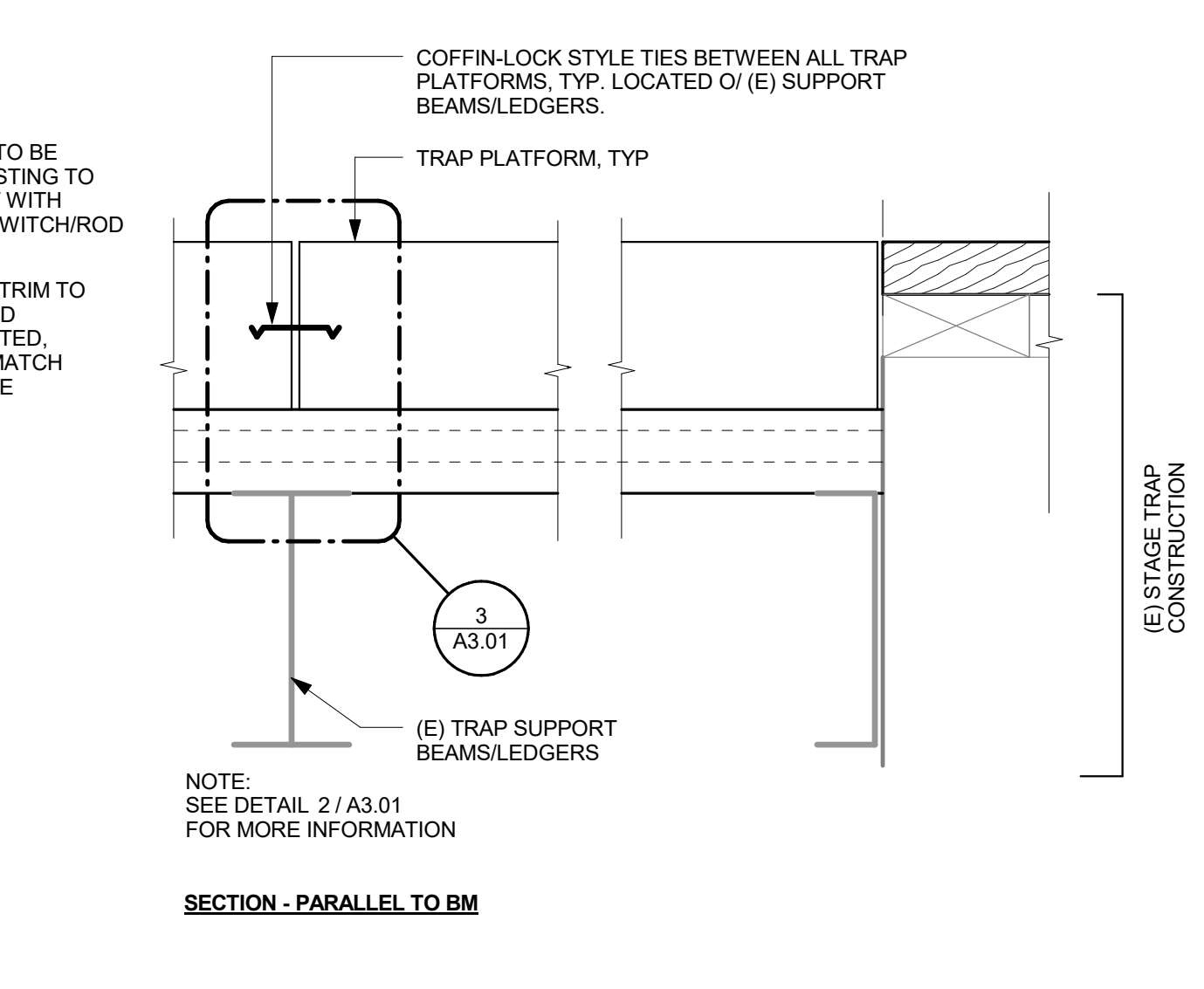
4 STAGE TRAP SECTION B SCALE: 3" = 1'-0"
