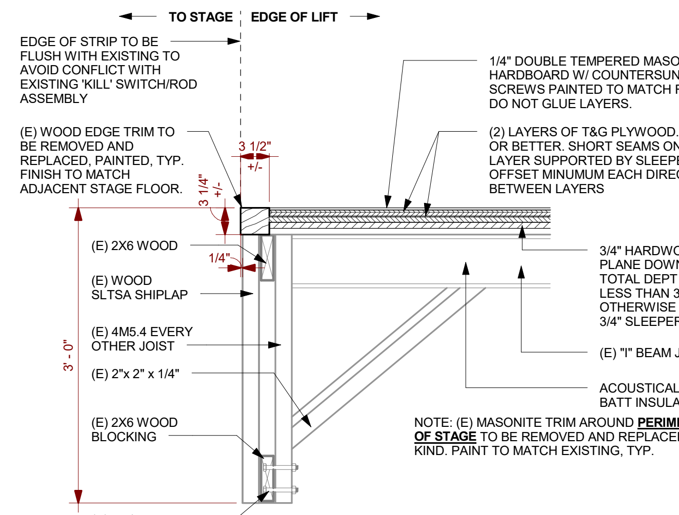
7 STAGE LIFT DETAIL A SCALE: 1" = 1'-0"
